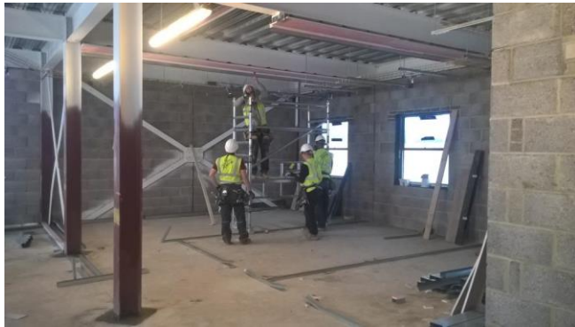
Internal walls of offices at Larkhill being constructed using plasterboard on metal studs
